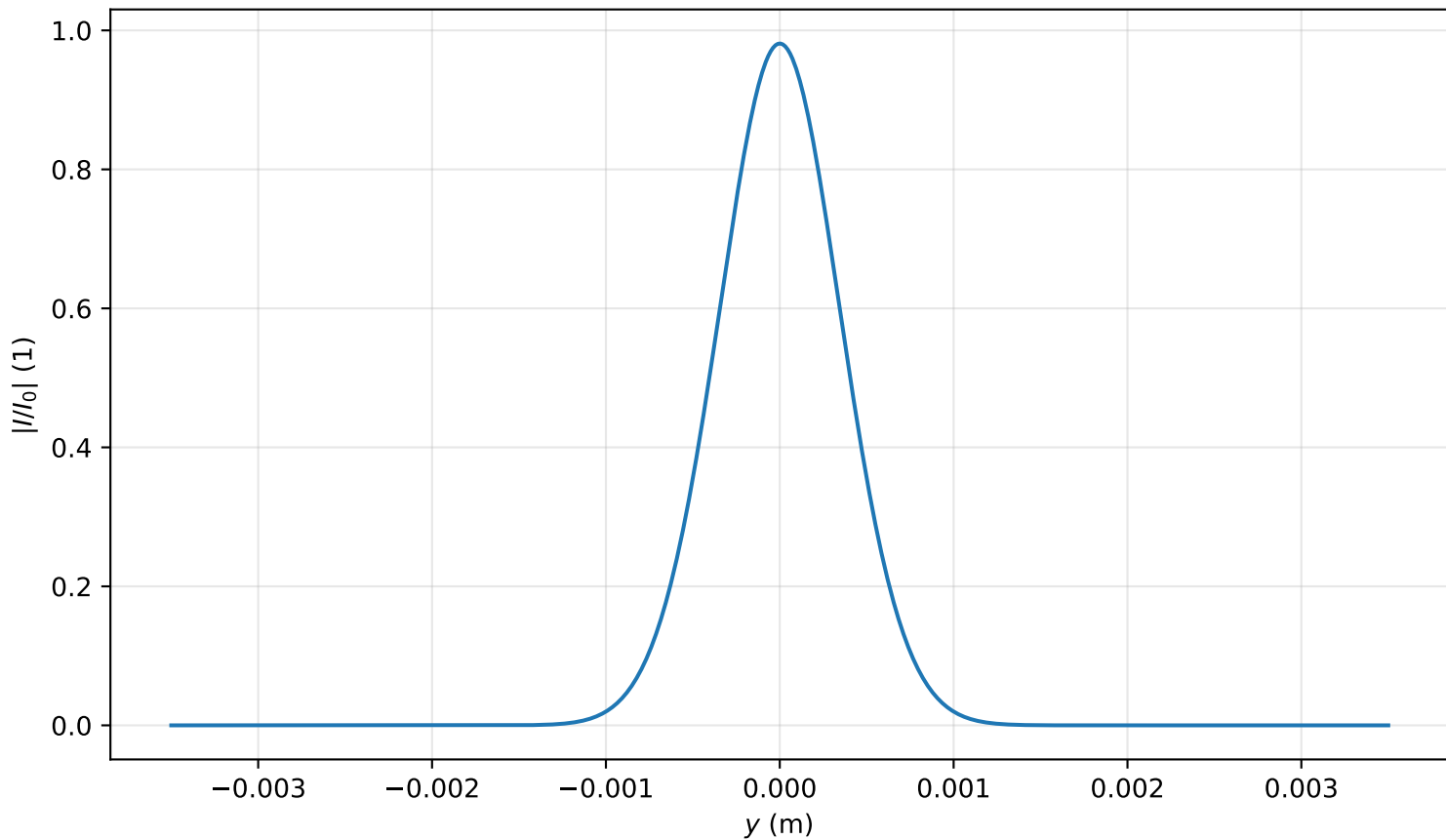
Intensity profile I(x=0, y, z=0.478)/I_0 , \text{Pin}=0.2\text{Pcr} , artificial time
